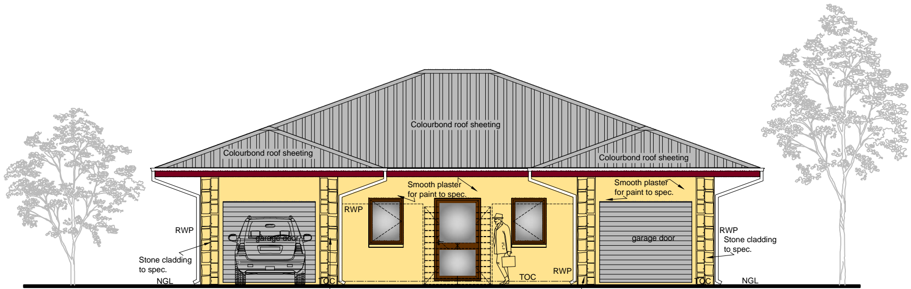
ELEVATION 1-1
